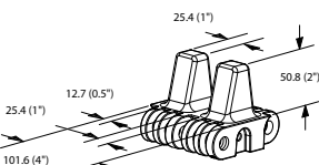
T2 dimensions
