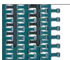
Supergrip for inclined conveying; Standard 100% rubber.
