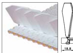
Sideguards for 1500-series imperial
